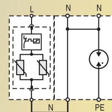
PROTEC B2SR 25/xxx (1+1)
