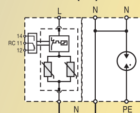
PROTEC B2SR 25/xxx (1+1)
