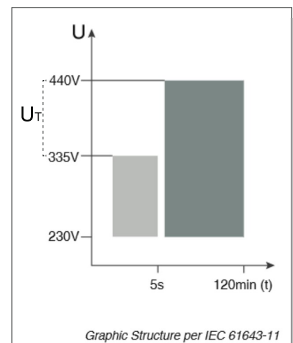
Graphic Structure per IEC 61643-11
